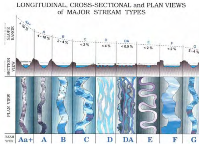
Figure 4: David Rosgen’s Diagram of Major Stream Types.
